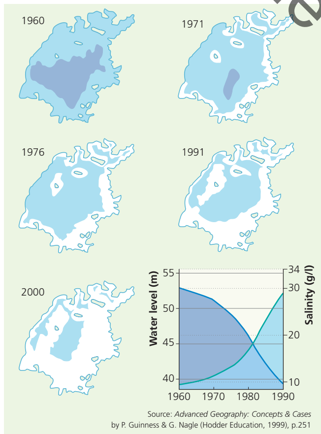
Figure 1.27 The changing hydrology of the Aral Sea
