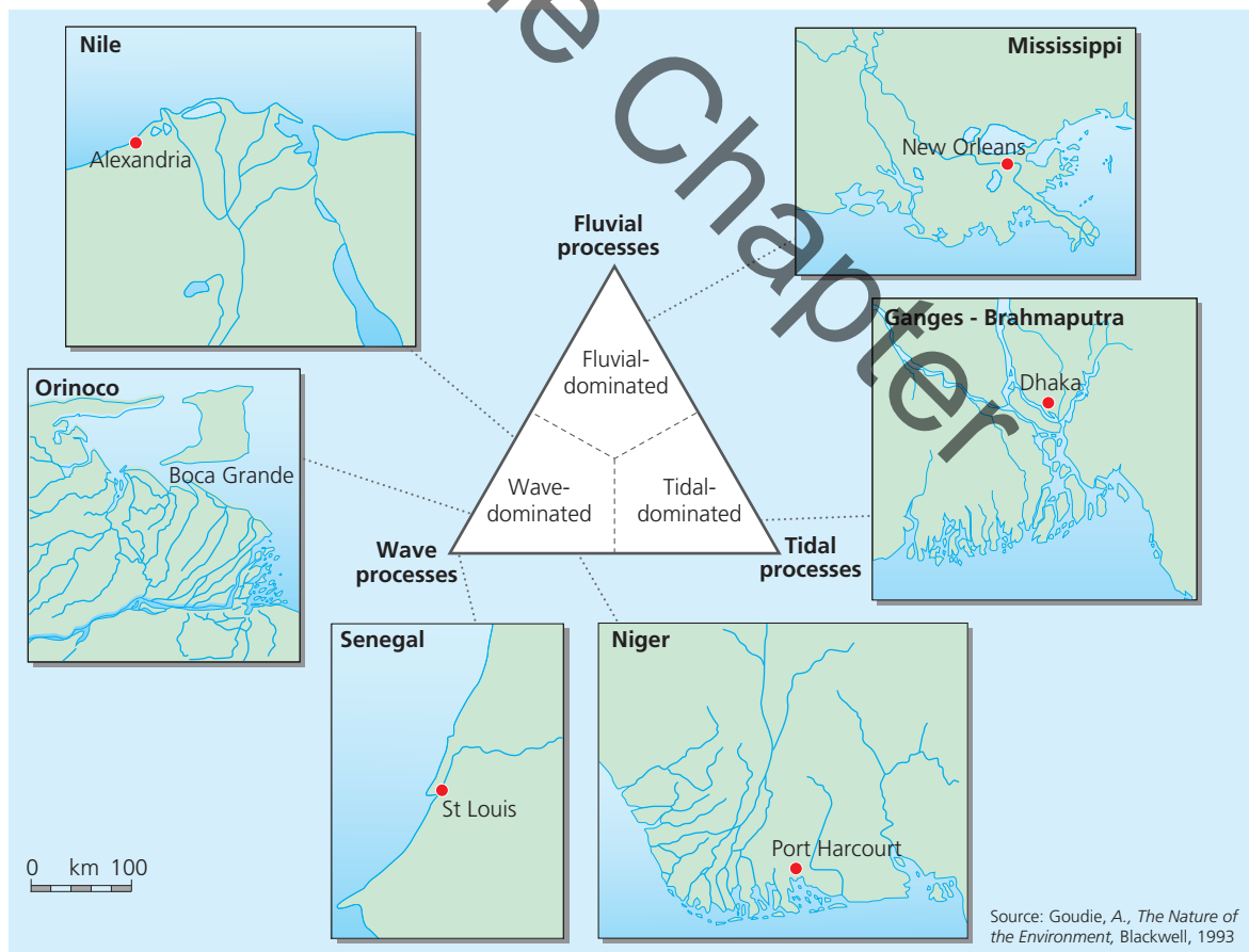
Figure 1.23 River delta shapes related to river, wave and tidal processes
