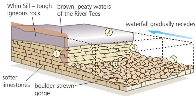
Figure 1.17 Waterfall formation
