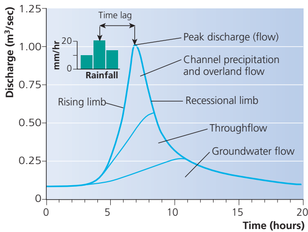
Figure 1.8 A simple hydrograph
