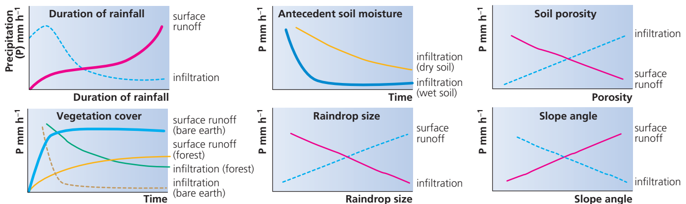
Figure 1.6 Factors affecting infiltration and surface runoff
