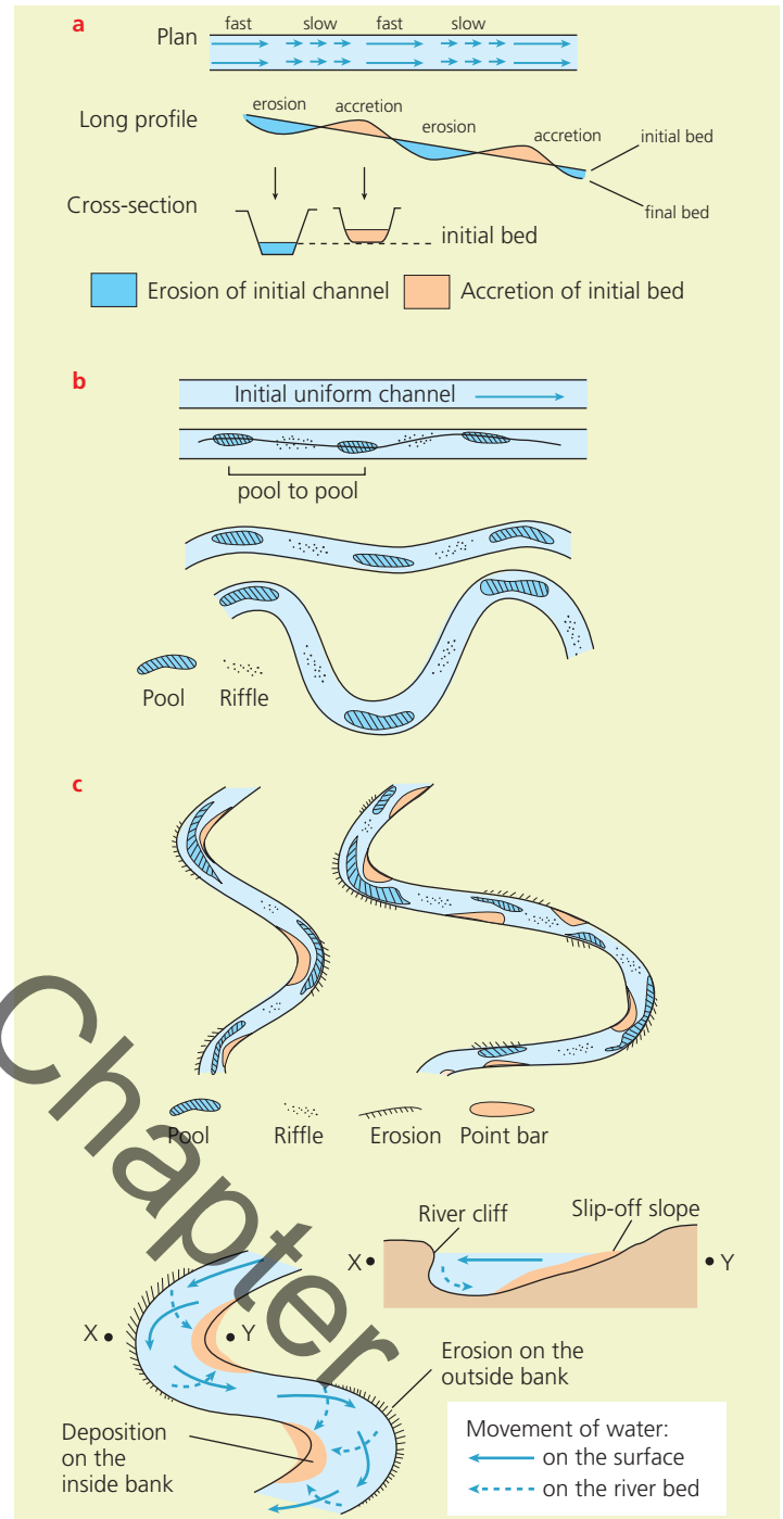
Figure 1.15 Meander formation
