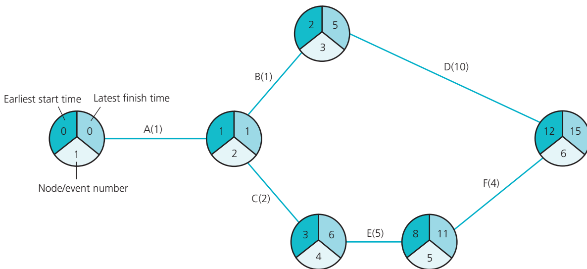
▲ Figure 3.25 Critical path analysis (CPA)
