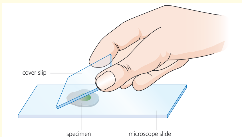
▲ Figure 1.9 How to make a light microscope slide.
