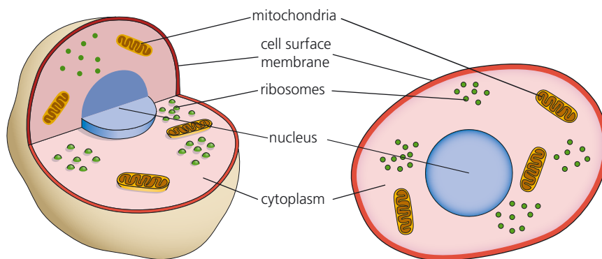
▲ Figure 1.6 A generalised animal cell as seen with a microscope (magnified \times 4800 ) and as three- and two-dimensional diagrams.
