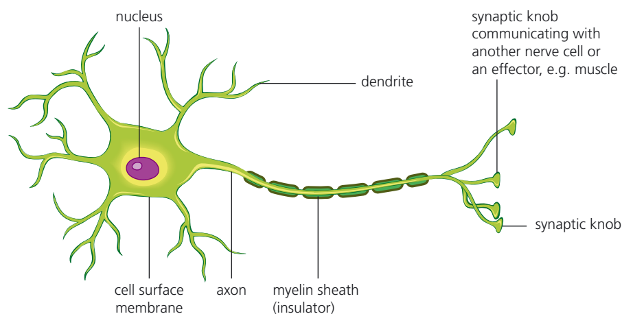
▲ Figure 1.11 The parts of a nerve cell.
