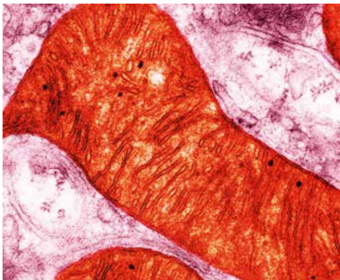
▲ Figure 1.20 (a) A three-dimensional image of an ant's head taken with a scanning electron microscope. (b) A two-dimensional image of a mitochondrion taken using a transmission electron microscope.
