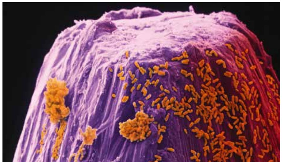
▲ Figure 1.5 Prokaryotic bacterial cells seen on a pinhead.
