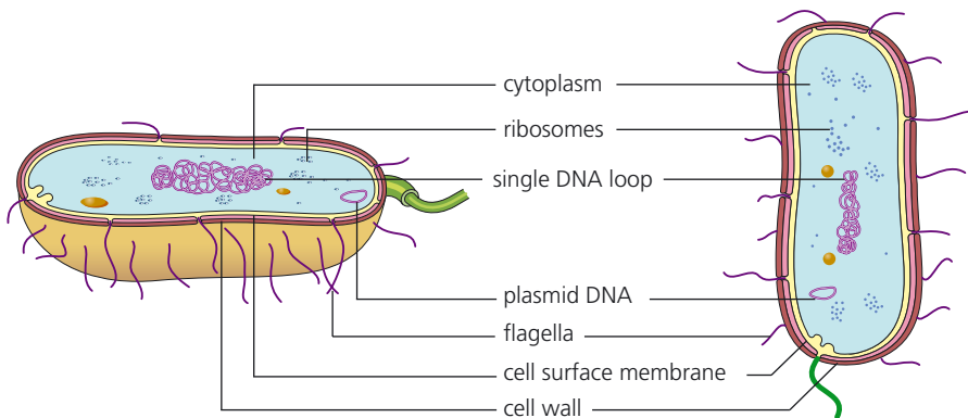
▲ Figure 1.4 A bacterial cell as seen with a microscope (magnified \times 20\,000 ) and as three- and two-dimensional diagrams.
