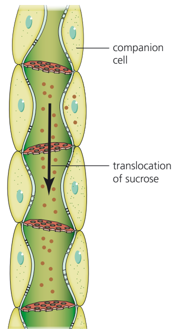
▲ Figure 1.16 The parts of a phloem tube.
