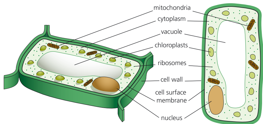
▲ Figure 1.7 A generalised plant cell as seen with a microscope (magnified \times 2800 ) and as three- and two-dimensional diagrams.
