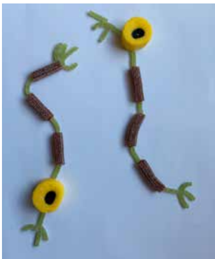
▲ Figure 1.12 A model of a eukaryotic cell made from sweets.
