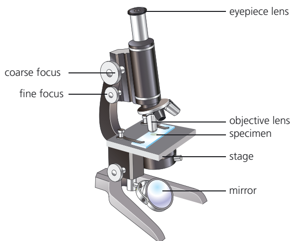
► Figure 1.18 A labelled diagram of a light microscope.
