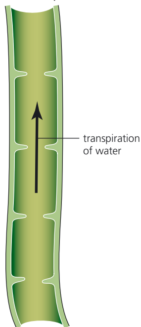
▲ Figure 1.15 The parts of a xylem tube.
