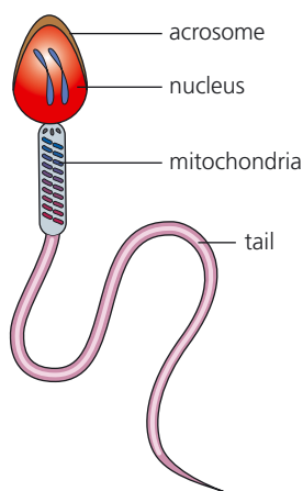
▲ Figure 1.10 The parts of a sperm cell.
