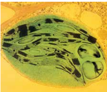
▲ Figure 1.8 The structure of a chloroplast (magnification about \times 15000 ).
