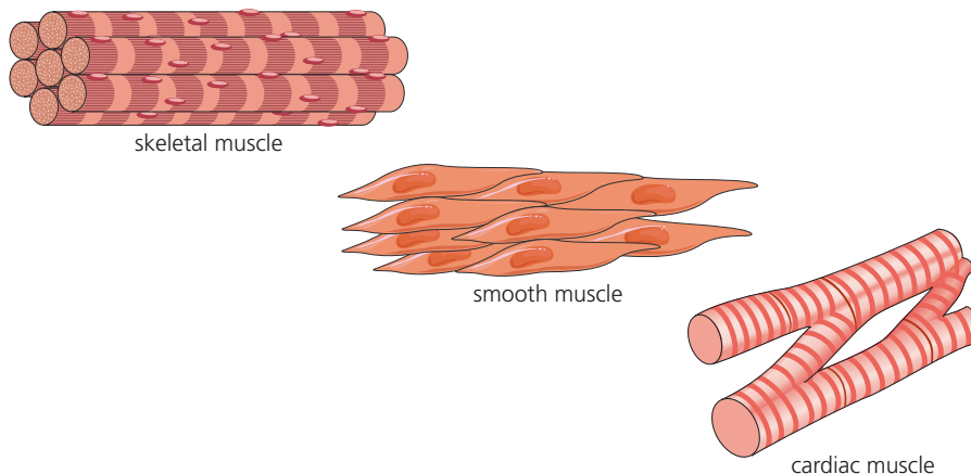
▲ Figure 1.13 The three types of muscle.
