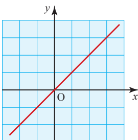
(b) Increasing for all values of x
