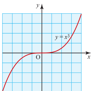
(c) Increasing for some values of x (all except x = 0 )
